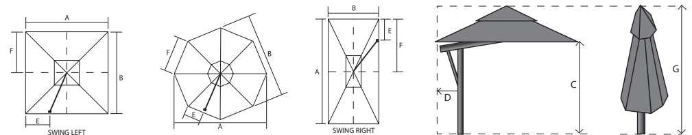
TROPICCOVER - MODELS, SHAPES AND SIZES - all measurements are approximate in mm
