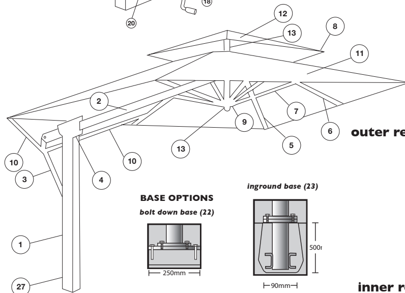
bolt down (22)
